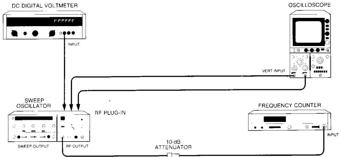
Figure 5-2. Adjustment Test Setup
