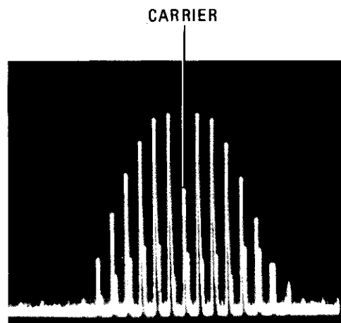
Figure 4-19. Spectrum Analyzer Display of First Carrier-null with 2.1 MHz Modulation Frequency
